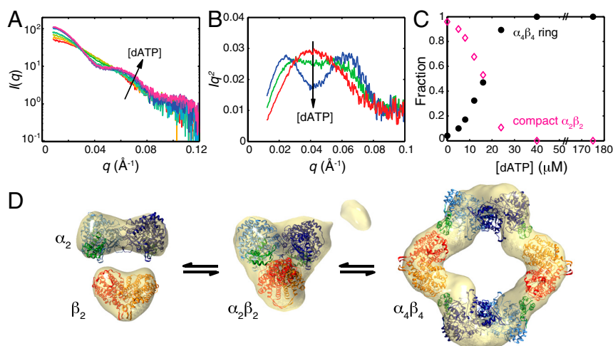
Fig. 4. SAXS investigation of the transition between lower and higher order structures of E. coli class Ia RNR. (A) Scattering curves measured as 0–175 \mu\text{M} dATP was titrated into a 6 \mu\text{M} solution of \alpha_2 and \beta_2 in the presence of 1 mM CDP (red to violet) display isointensity points, suggesting a two-state transition. (B) Kratky representations of the scattering curves ( I(q^2) vs. q ) at 0 \mu\text{M} (red), 12 \mu\text{M} (green), and 40 \mu\text{M} (blue) dATP show a transition from a compact globular state, as indicated by the monomodal peak, to a large nonglobular state, indicated by a bimodal curve (36). (C) Fitting linear combinations of the \alpha_2\beta_2 docking model (15) and the \alpha_4\beta_4 ring to the titration data provided relative fractions of the two states. (D) Ab initio SAXS reconstructions of free subunits aligned with deposited crystal structures (5, 39), a compact \alpha_2\beta_2 state aligned with the proposed docking model (15), and the \alpha_4\beta_4 ring aligned with the crystal structure (SI Appendix, Tables S2 and S3, and Fig. S10). The small additional density observed in the molecular envelope of \alpha_2\beta_2 can be explained by the presence of approximately 3% \alpha_4\beta_4 (Fig. 4 C ).
